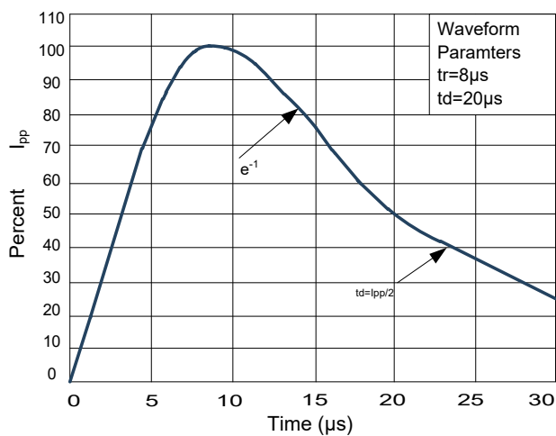
Figure3: Pulse Waveform
